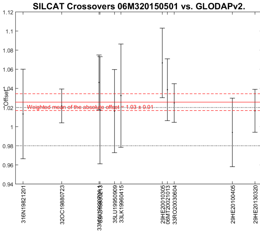
Figure 4: This figure shows the collected results for all crossovers for silicate for cruise 06M320150501 vs. GLODAPv2. The generally high values (i.e. above 1) indicate that a downward adjustment for silicate could be necessary.
