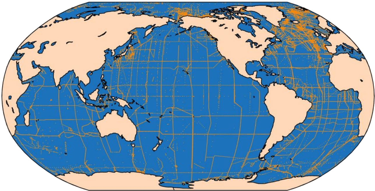
Figure 1: Map of stations in GLODAPv2 published in 2016.
