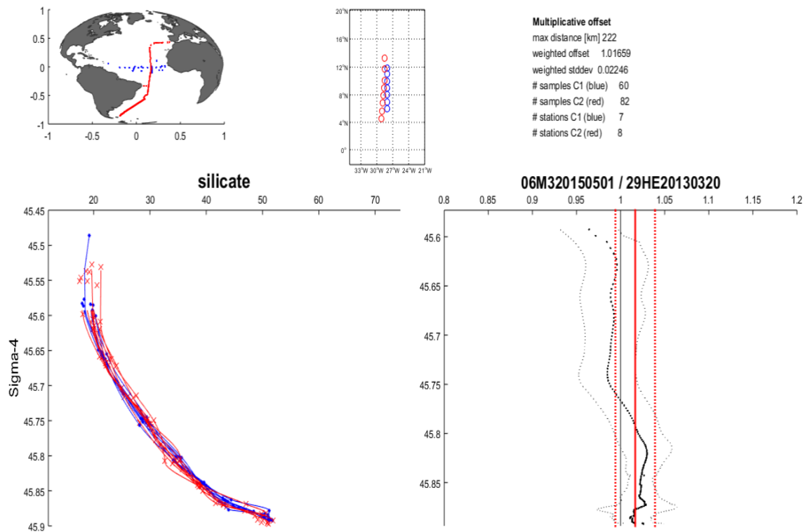
Figure 3: Example of a crossover for a cruise in the tropical Atlantic, the cruise in blue is a new cruise that is compared to a cruise from GLODAPv2 (in red).
